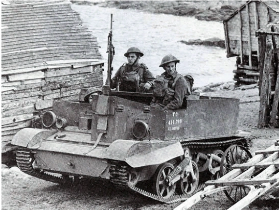
Universal Carrier Mk II
